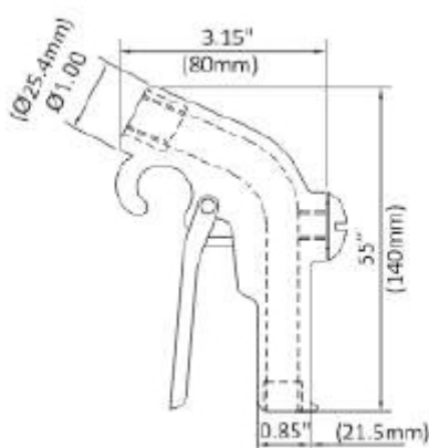
Easy Grip Safety Gun
